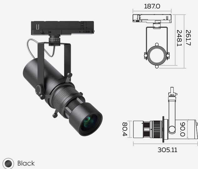
Standard Version (Unit:mm)
